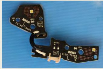
PCB of the positioning light
