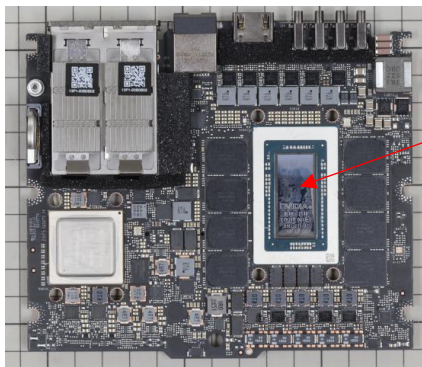
Main PCB
