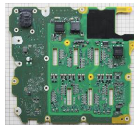
PCB(Bottom View)
