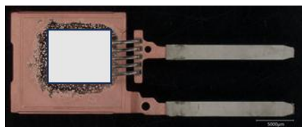
TO-247PLUS-4 IMYR140R006M2H
